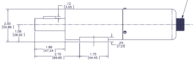
RESOLVER SHOWN IN ZERO-DEGREES POSITION, WITH KEY PERPENDICULAR TO BASE
